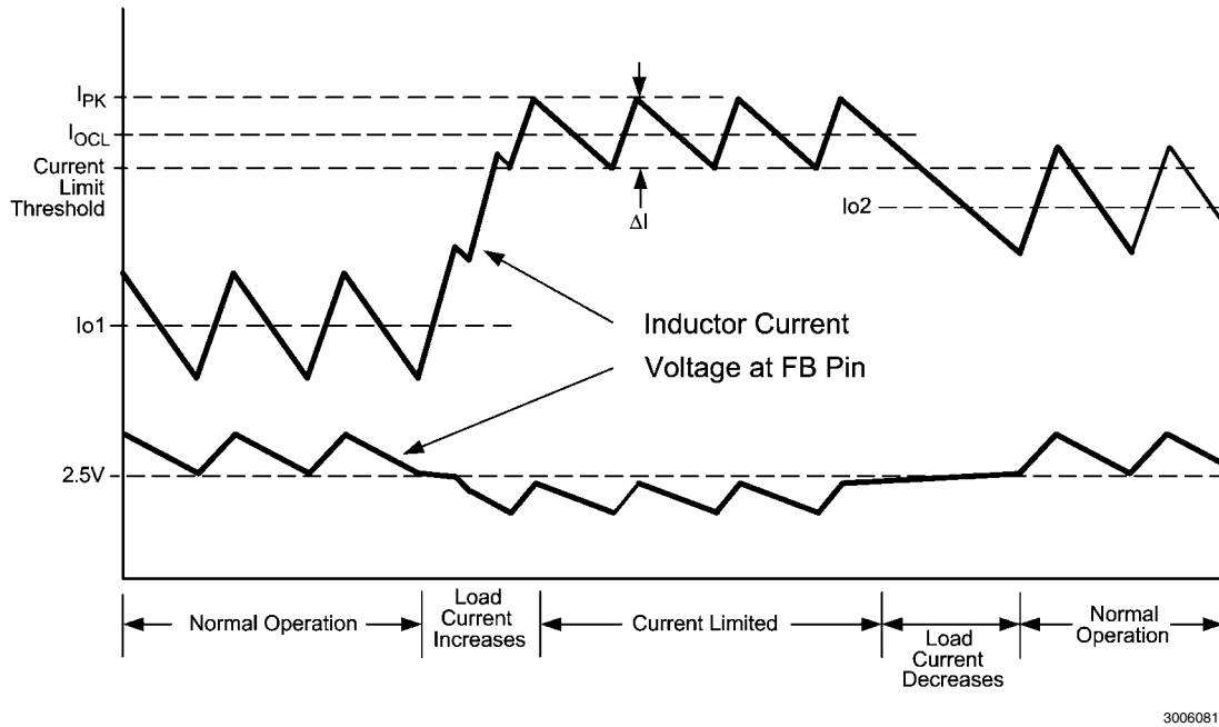
FIGURE 2. Inductor Current - Normal and Current Limit Operation
